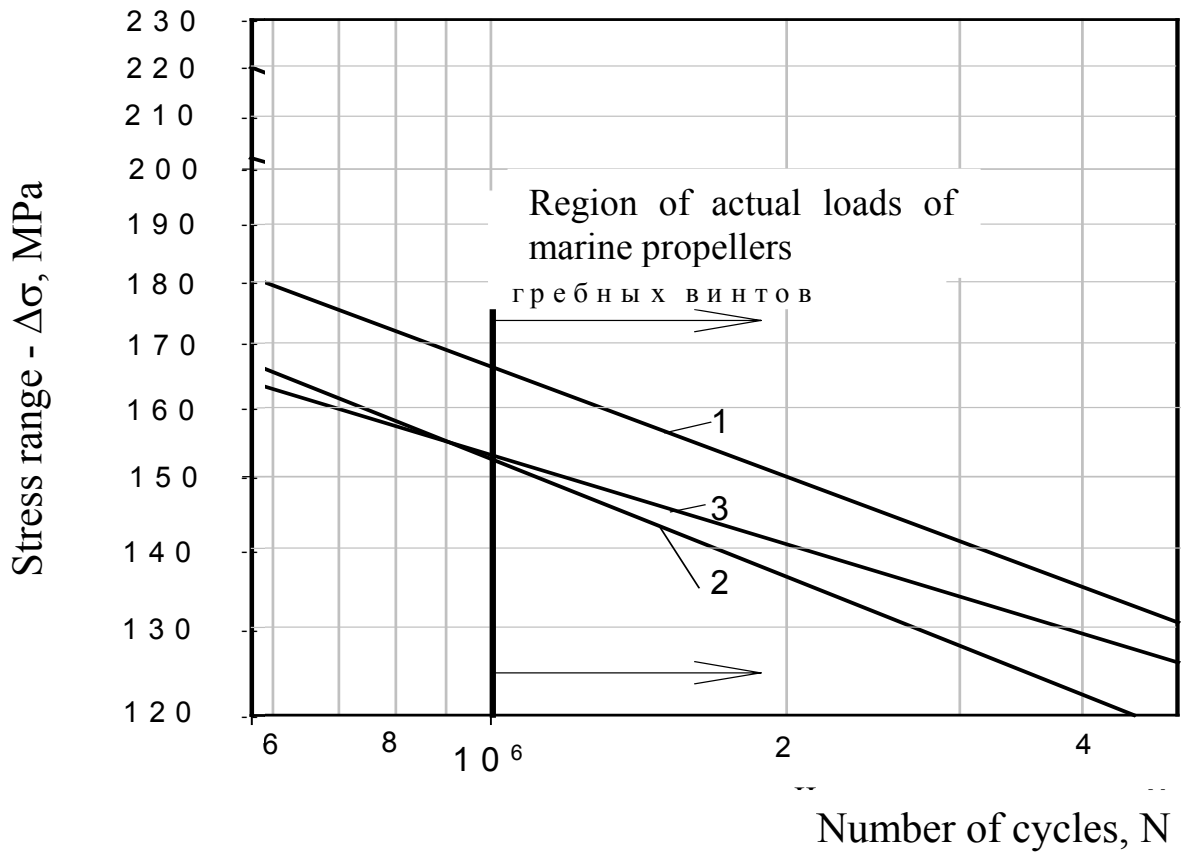
Fig. 16 Fatigue curves for bronze specimens (axial loading r = 0,5 ) in synthetic salt water: 1 – base metal; 2 – deposition plus heat treatment; 3 – deposition plus UIT
