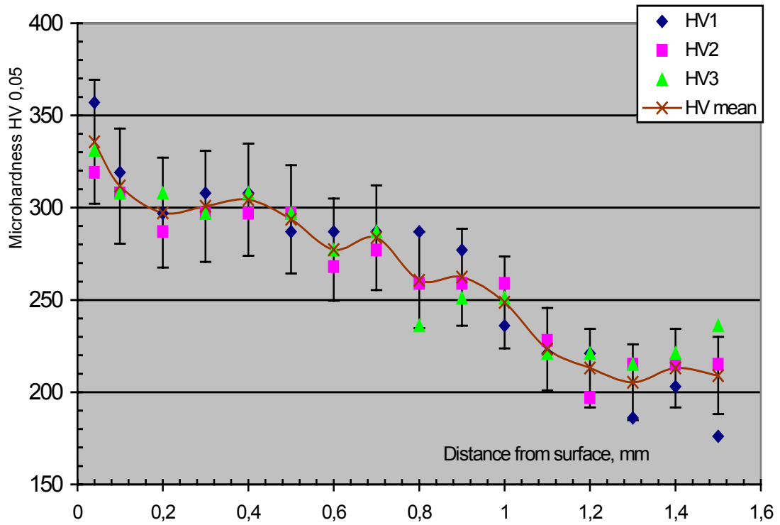
Fig. 26 Specimen No. 3 – deposited metal treated by manual UIT followed by finish with Durex disk
