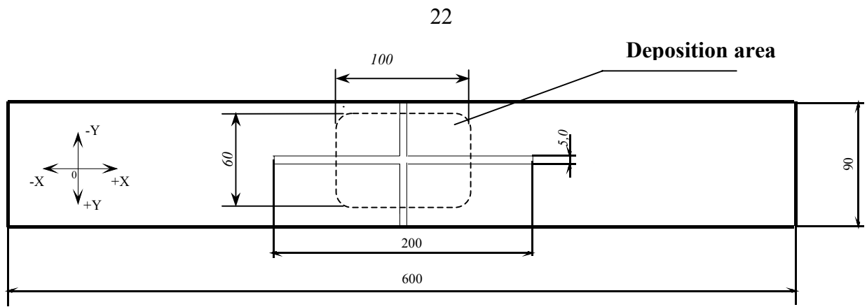
Fig. 11 Layout of areas for measurement of specimen surface residual stresses
