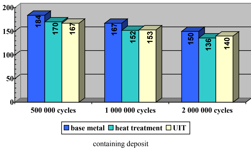
Fig. 17 Effect of heat treatment and UIT on corrosion cyclic life of plate in bronze BrA9Zn4N4
