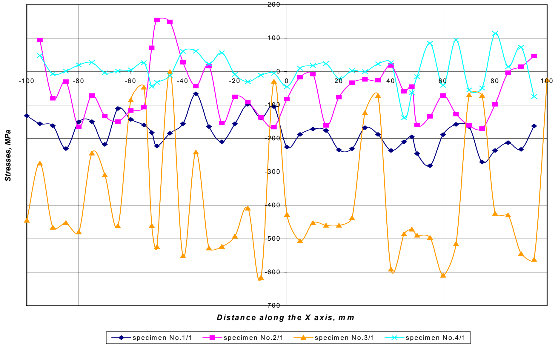
Fig. 13 Diagram of residual stress distribution along the X axis in transverse direction
