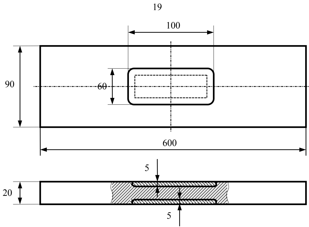
Fig. 6 Corrosion fatigue test specimens
