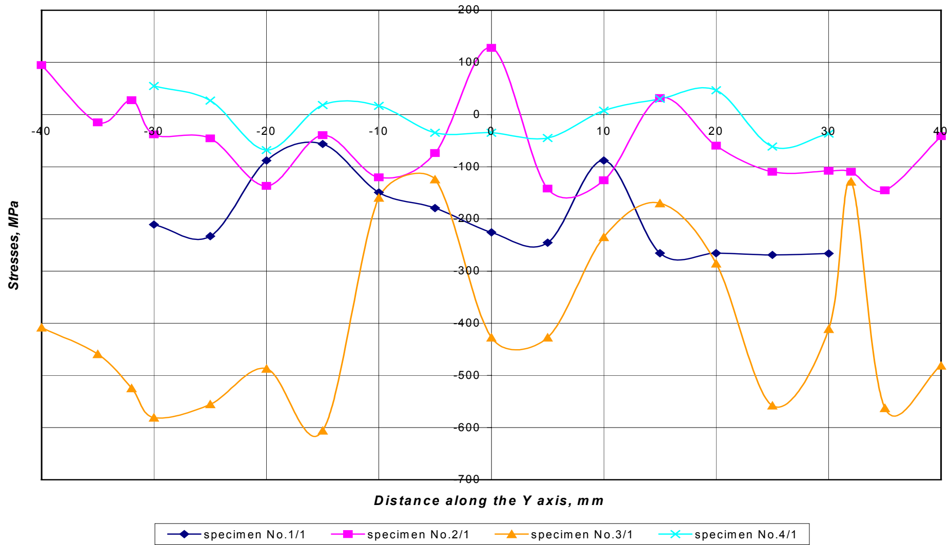
Fig. 15 Diagram of residual stress distribution along the Y axis in transverse direction
