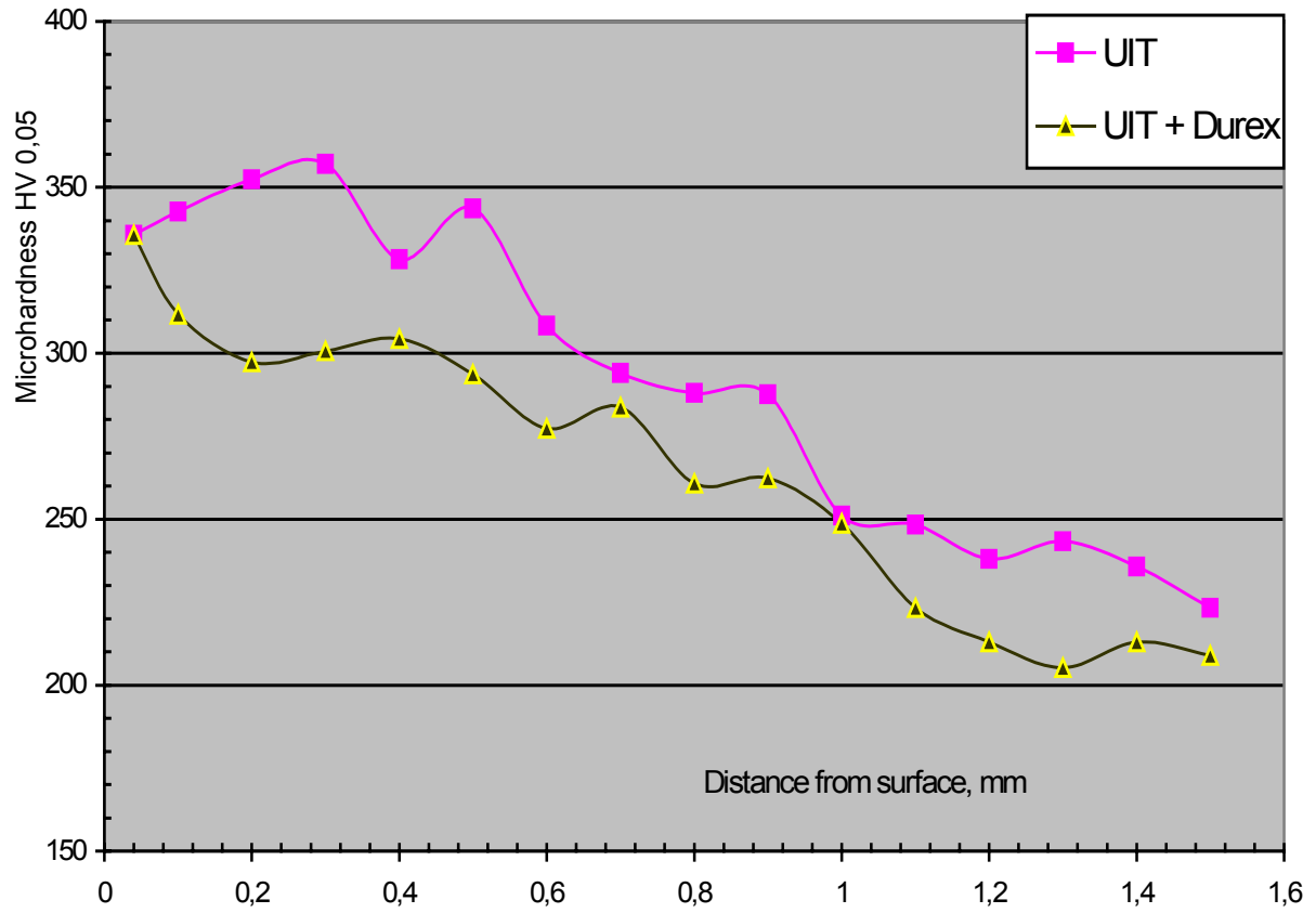
Fig. 30 Microhardness (HV 0,05 mean) of deposited metal after various treatments
