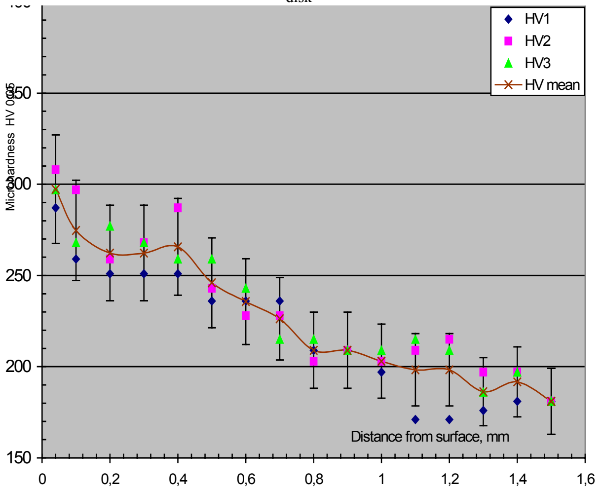
Fig. 27 Specimen No. 4 – base metal treated by manual UIT followed by finish with Durex disk
