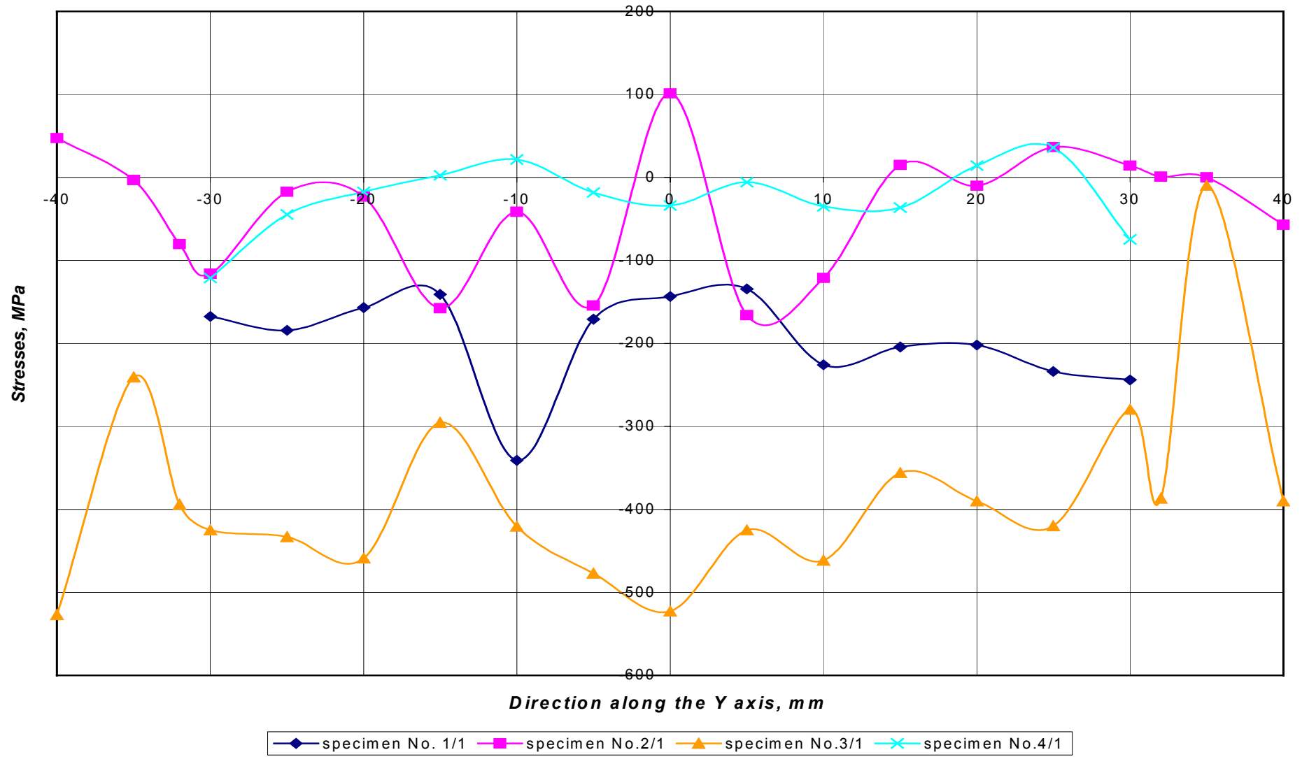
Fig. 14 Diagram of residual stress distribution along the Y axis in longitudinal direction
