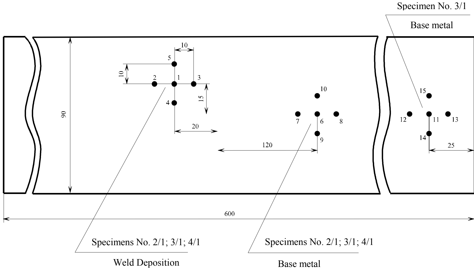
Fig. 10 Diagram of hardness measurement on bronze specimens
