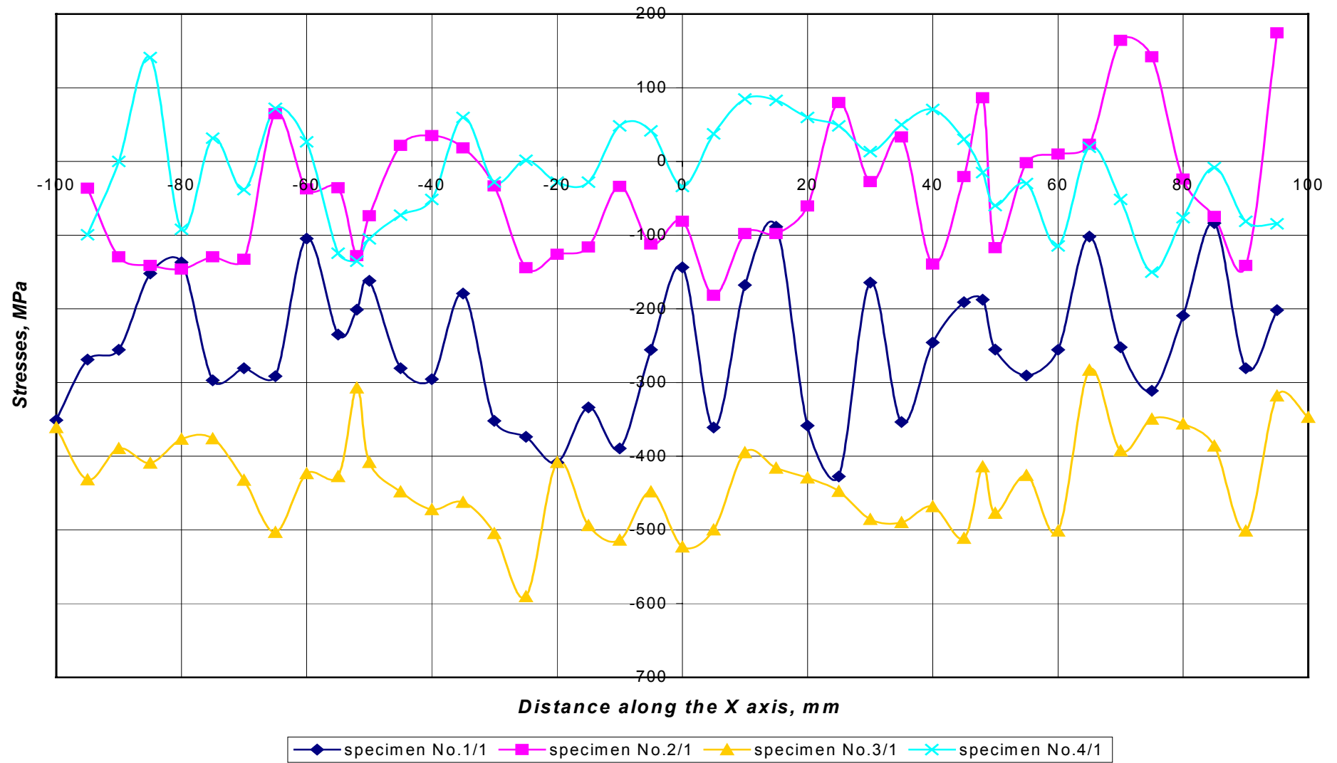
Fig. 12 Diagram of residual stress distribution along the X axis in longitudinal direction
